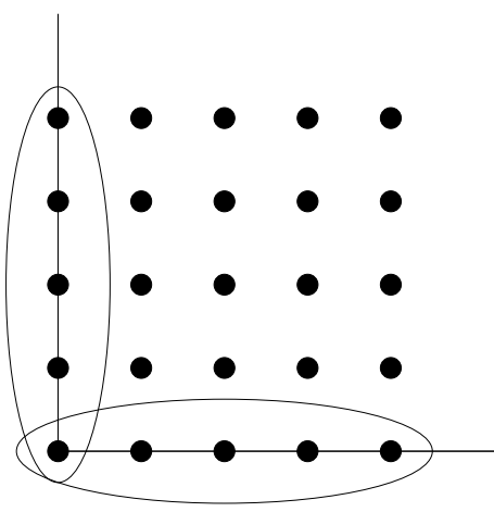
Figure 1: Example Numbers game problem: tests are points in a 2-d space. In Pareto-coevolution, all n^2 tests would be separate objectives. The two underlying objectives (marked by ellipses) are more compact, yet provide equivalent information.
